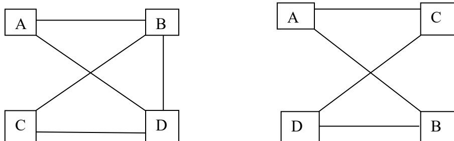
Undirected Graph
