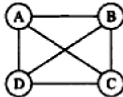
Connected Graph
