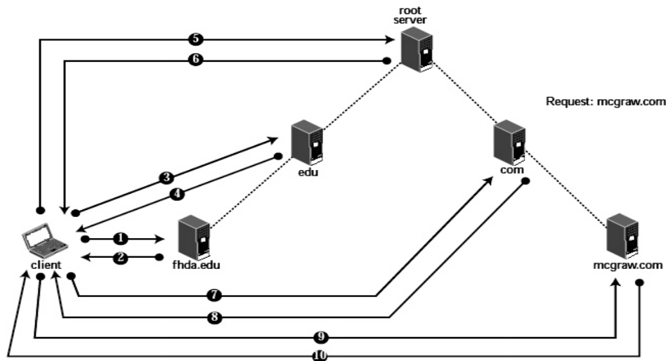
Figure 14.7: Iterative resolution [4]
