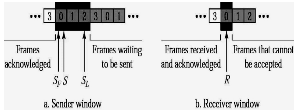
Figure 5.22: Control variables [2]
