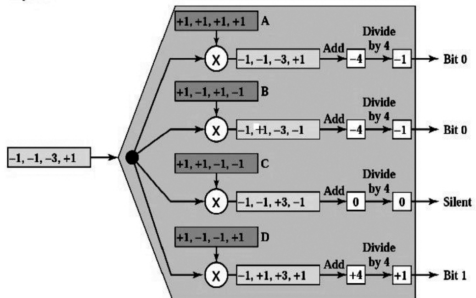
Figure 6.25: CDMA demultiplexer [1]
