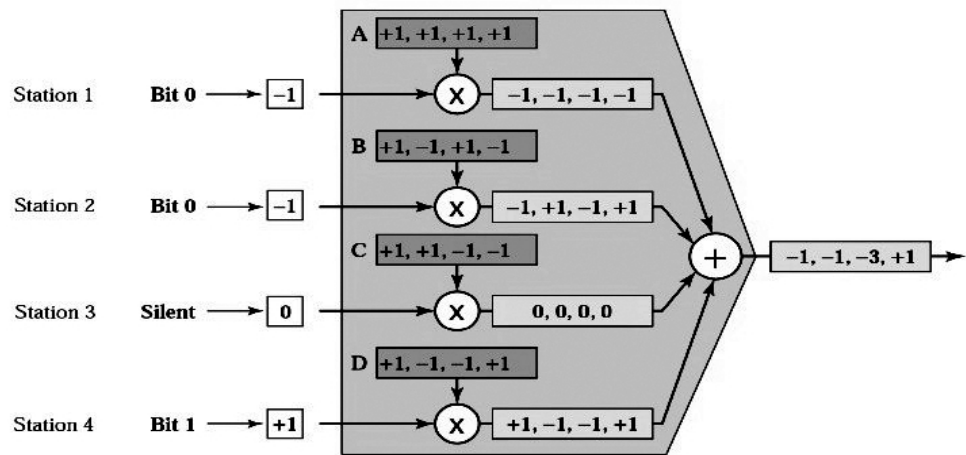
Figure 6.24: CDMA multiplexer [1]
