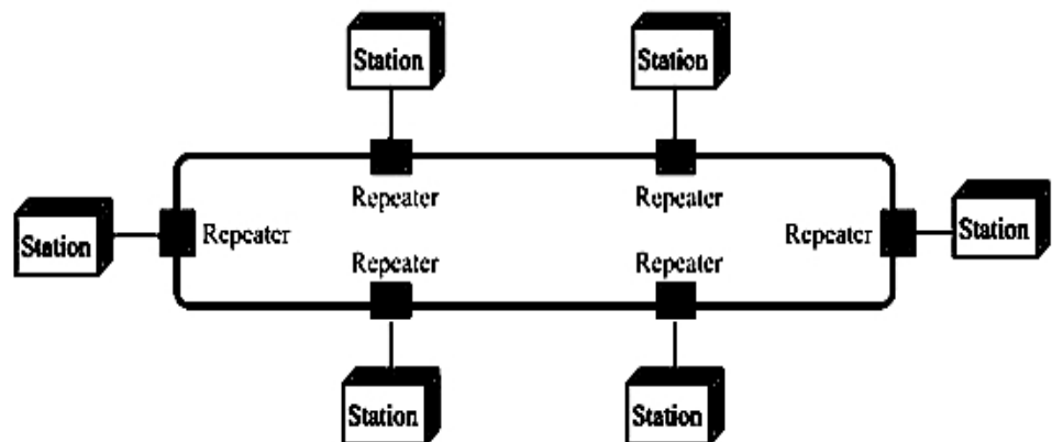
Figure 1.7: A ring topology connecting six stations [1]
