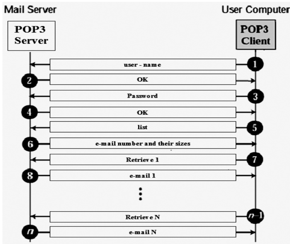
Figure 14.18: POP3 [6]
