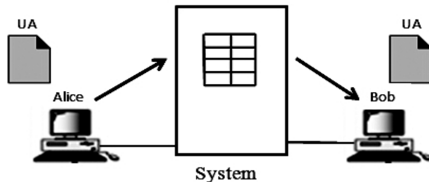
Figure 14.9: First scenario [5]
