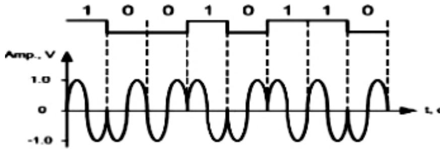
Figure 3.5. Phase Shift Keying [6]
