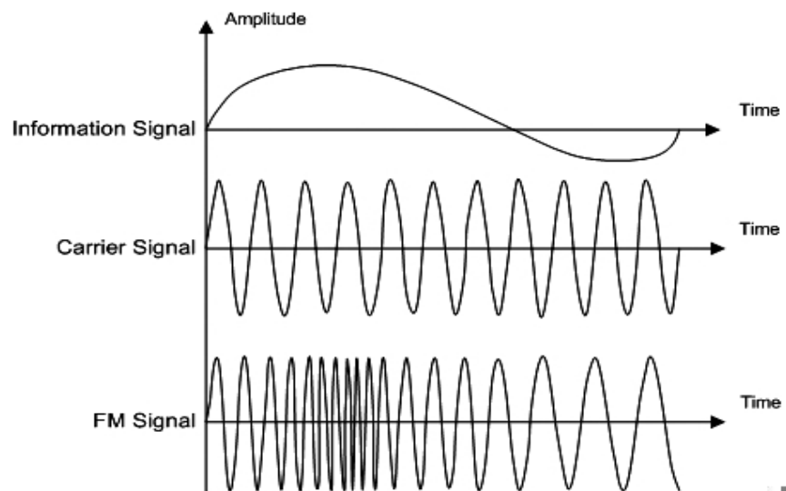
Figure 3.14: Frequency Modulation [10]
