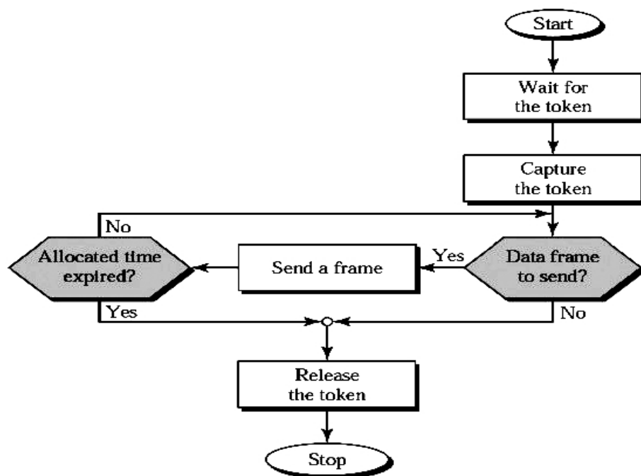
Figure 6.15: Token-passing procedure [1]
