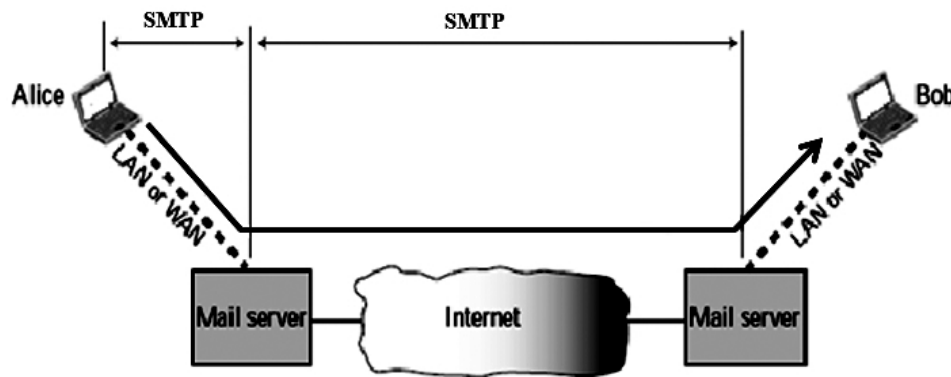
Figure 14.16: SMTP range [6]
