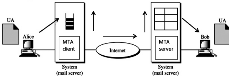
Figure 14.10: Second scenario [5]
