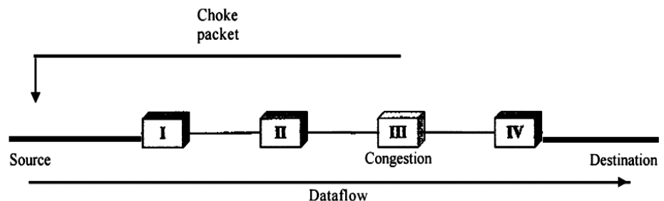
Figure 11.8: Choke packet [4]
