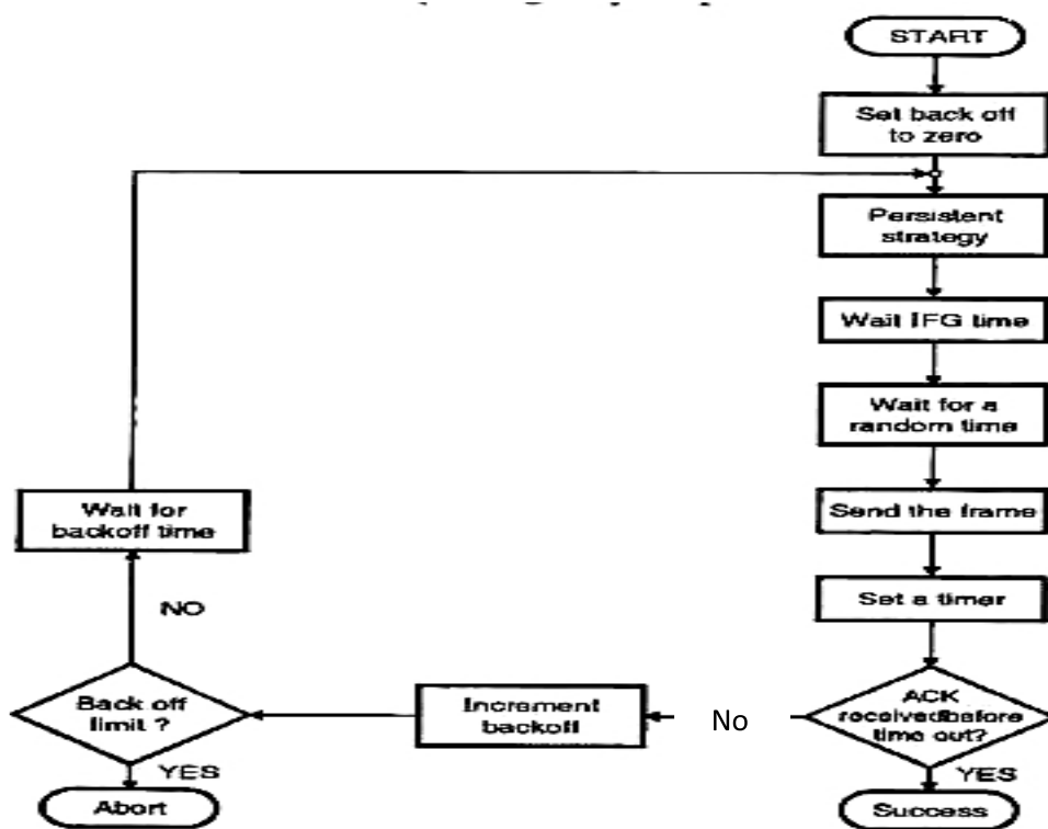
Figure 6.10: CSMA/CA procedure [1]
