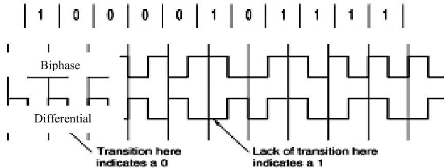
Figure 3.7: Biphase encoding schemes [8]
