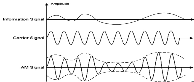
Figure 3.13: Amplitude Modulation [10]
