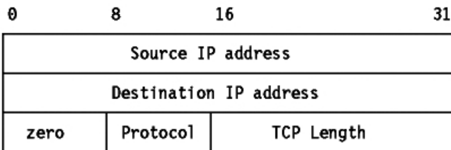
Figure 12.14: Pseudo-header [6]
