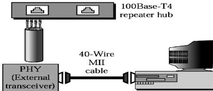
Figure 7.22: 100Base-T4 implementation [2]
