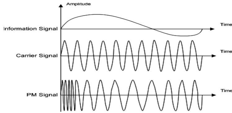
Figure 3.15: Phase modulation [10]
