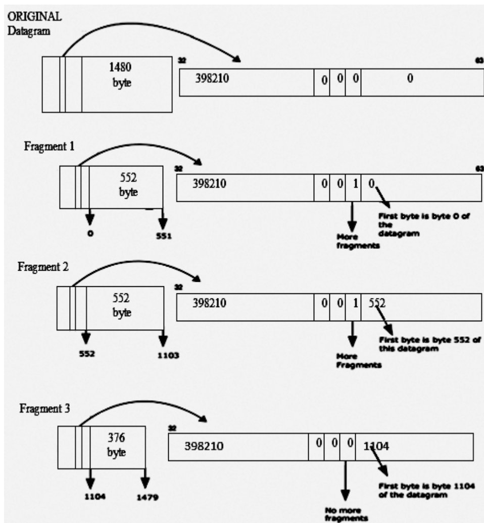
Figure 10.4: Packet fragmentation [2]
