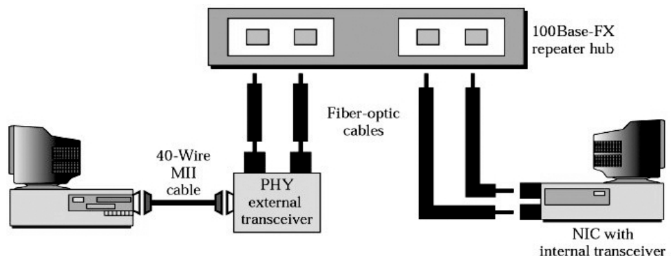
Figure 7.21: 100Base-FX implementation [2]
