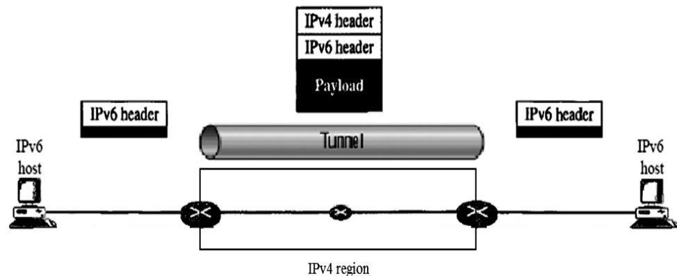
Figure 10.5: Tunneling strategy [3]
