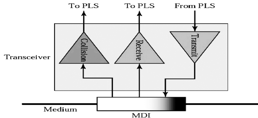
Figure 7.8: MAU (Transceiver) [2]
