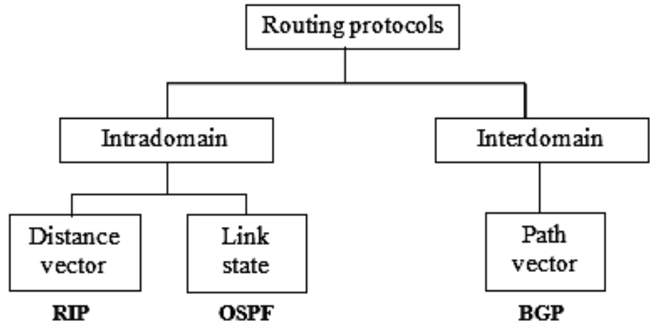
Figure 11.2: Routing protocols [2]
