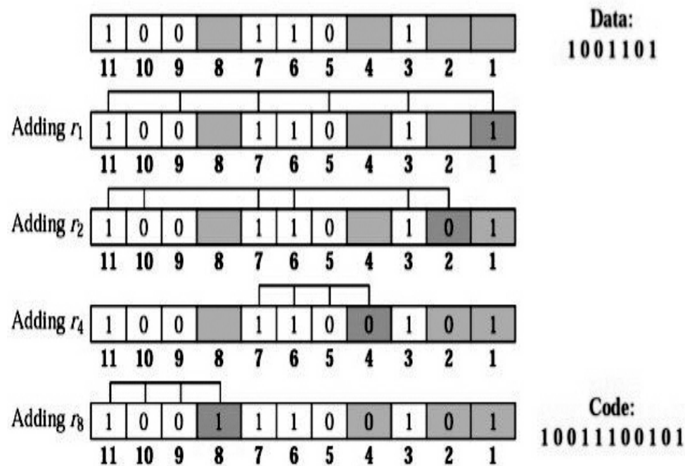
Figure 5.11: Redundancy bit calculation [1]
