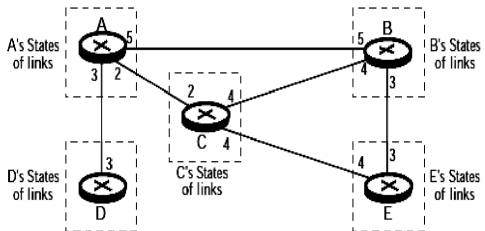
Figure 11.3: Link state knowledge [2]
