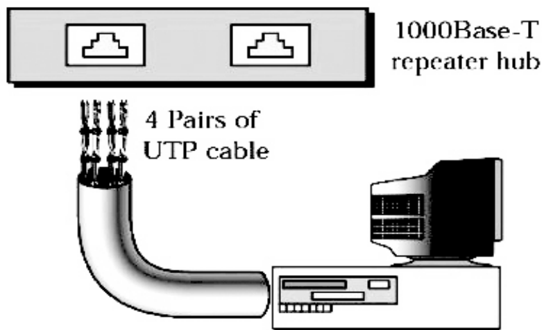
Figure 7.26: 1000Base-T implementation [2]
