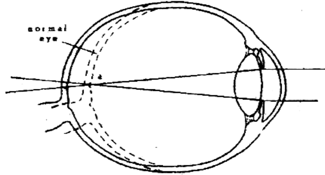
Fig. 2.3. Myopia (Nearsightedness)
