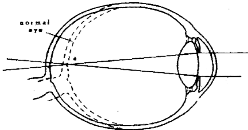
Fig. 2.3. Myopia (Nearsightedness)
